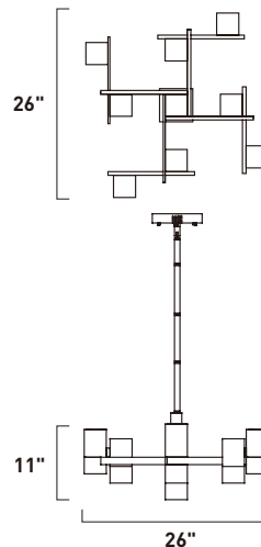
Frame diagram and overall measurements
