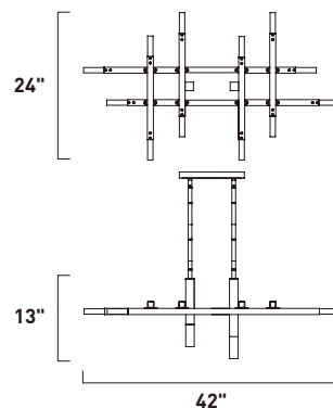
Frame diagram and overall measurements
