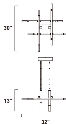
Frame diagram and overall measurements
