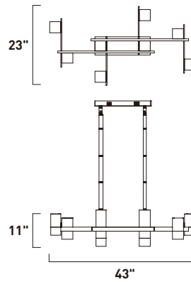
Frame diagram and overall measurements
